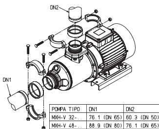
Bocche con giunti Victaulic Victaulic ports Victaulic-Anschlüsse Raccordi Victaulic Acoplamiento Victaulic 进出口卡箍
